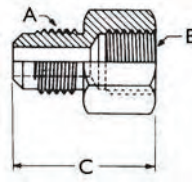
Half Union, Flare to NPTFI
