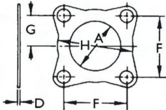
Flange with Flat Gasket Surface
