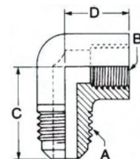
External Flare to NPTFI
