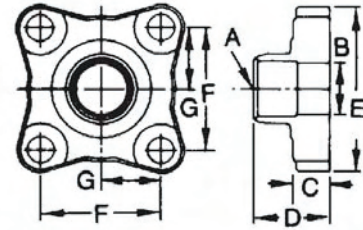
Flange with Groove
